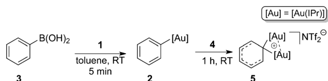
Scheme 1. Synthesis of gem -diaurated species 5 using the gold hydroxide 1 and the complex 4 .
